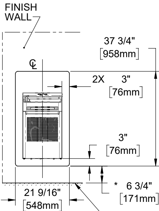
BP1201 FOR USE WITH ALL 1201 MODELS
