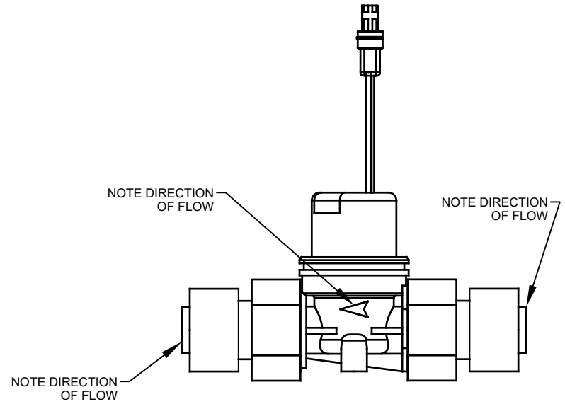
SOLENOID VALVE ASSEMBLY
