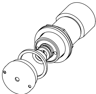
MODEL 5874PB PUSHBUTTON
