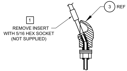
DETAIL A ROTATED 90° INTO VIEW
