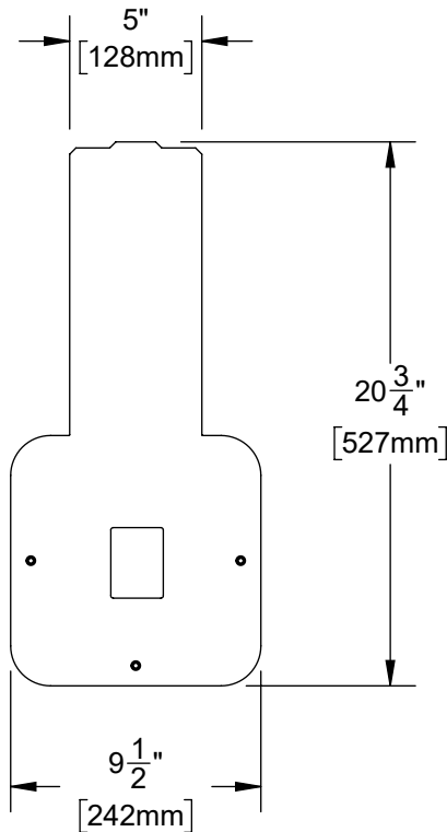
3655 PEDESTAL ARM BOTTOM ACCESS PLATE DETAIL
