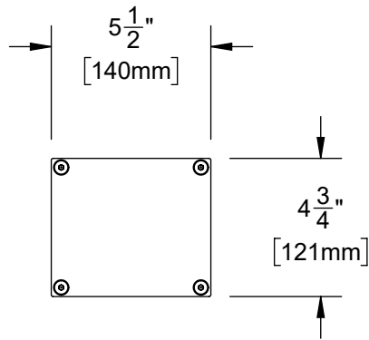
3652 SMALL ACCESS COVER PLATE DETAIL
