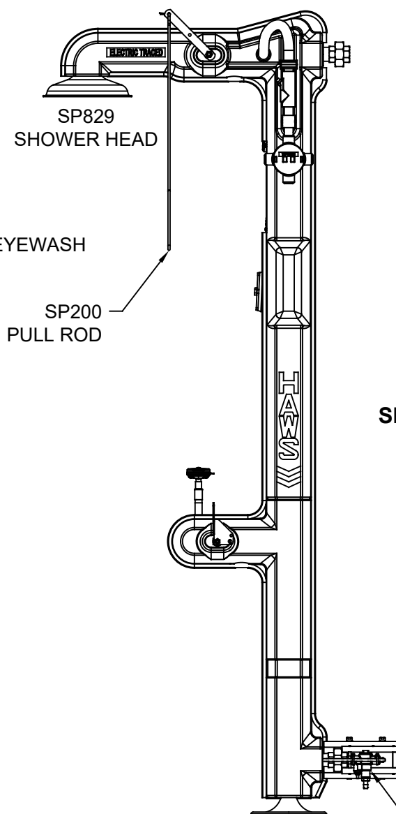
SIDE VIEW
