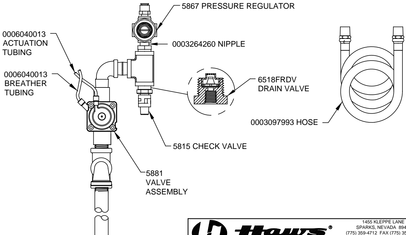
VRK3AV 1 DETAIL
