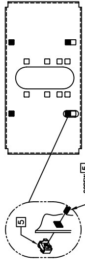
BOWL MOUNTING PATTERN DETAIL
