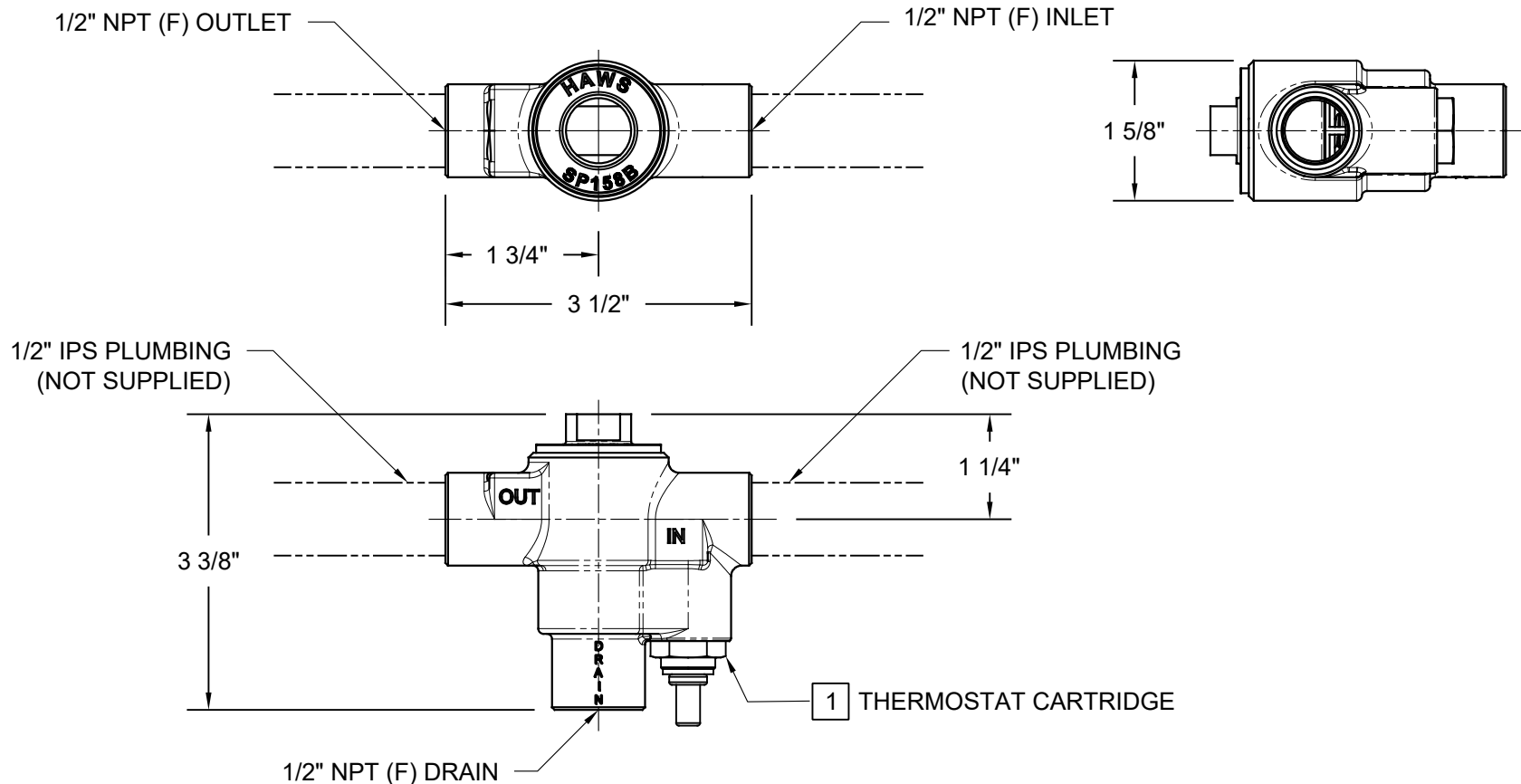
IN-LINE DRAIN INSTALLATION SHOWN (INLET AND OUTLET CONNECTED)
