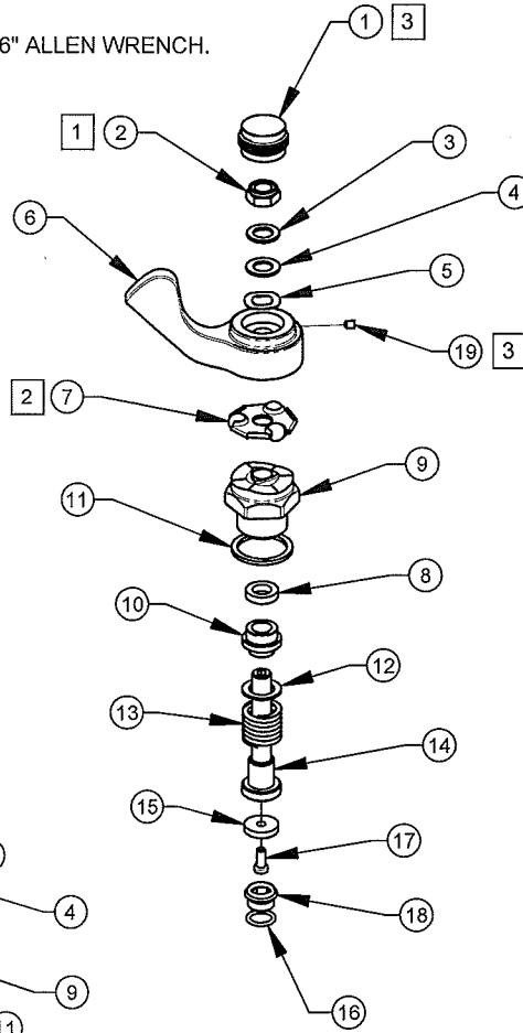
EXPLODED VIEW
